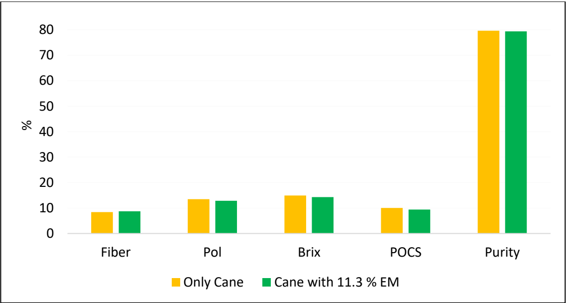
Figure 2.7 – Biochemical Parameters in burnt cane in a dirty field
